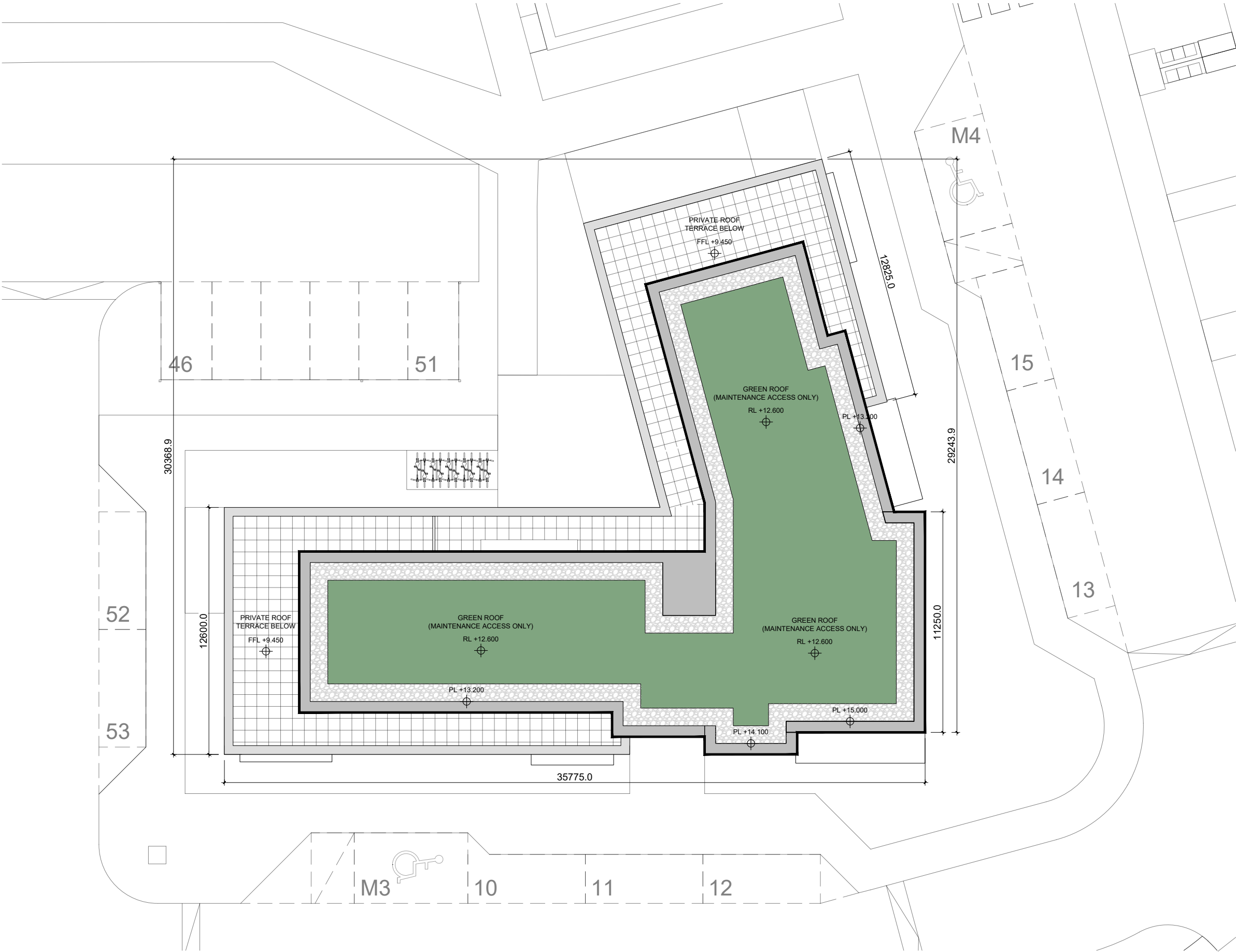
Apartment Block 02 - Roof Plan Scale 1:200
